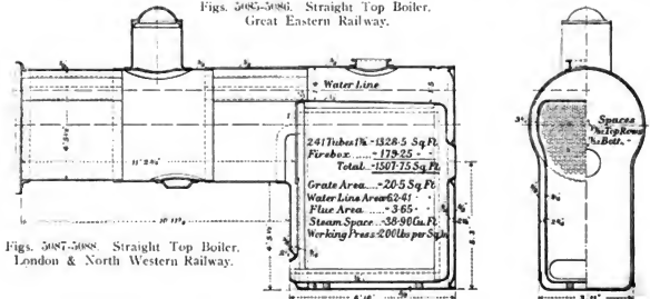
Figs. 5085-5086. Straight Top Boiler. Great Eastern Railway.
